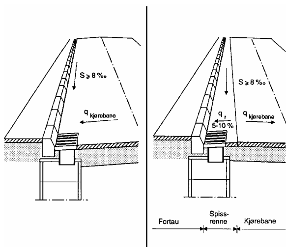
Figur 406.8 Enkel rennestein Figur 406.9 Spissrenne
