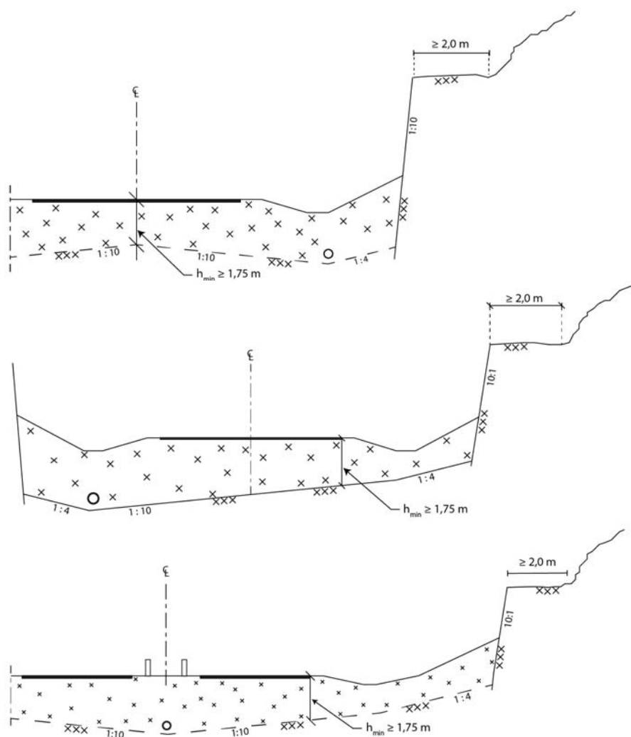
Figur 226.3 Dypsprengning
